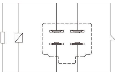
常开A型/Normally open A type
