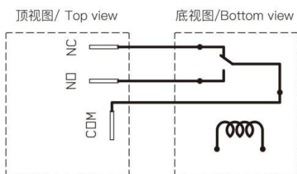
转换C型/Conversion C type
