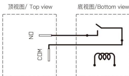
常开A型/Normally open A type
