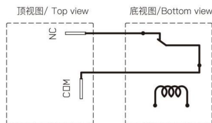
常闭B型/Normally closed B type
