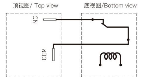
常闭B型/Normally closed B type
